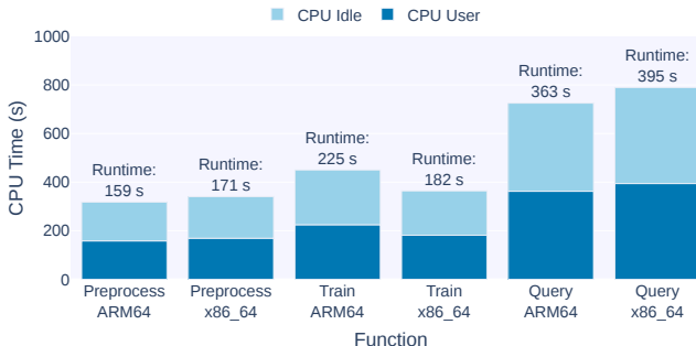
Figure 2: CPU time profile for the NLP pipeline
